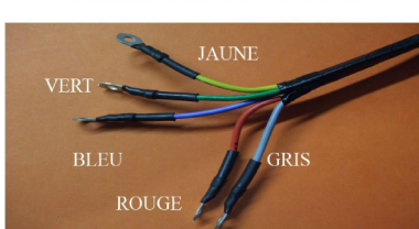
COMMODO CODE PHARE
